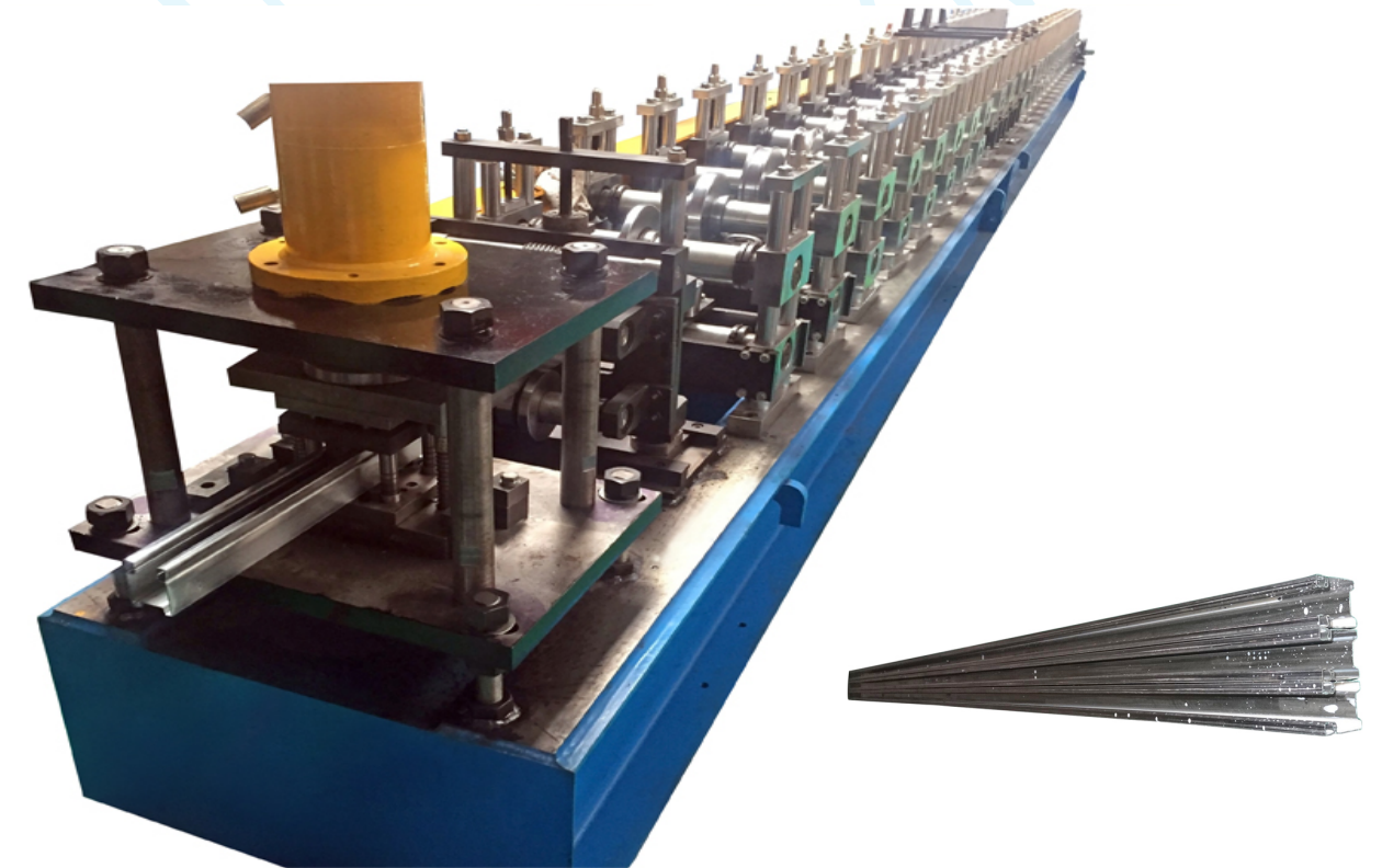
Roller shutter door roll forming machine
