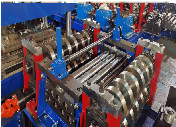
Leveling machine
