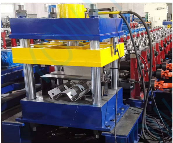
Hydraulic cutting
