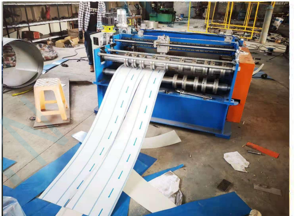
Oblique slitting machine
