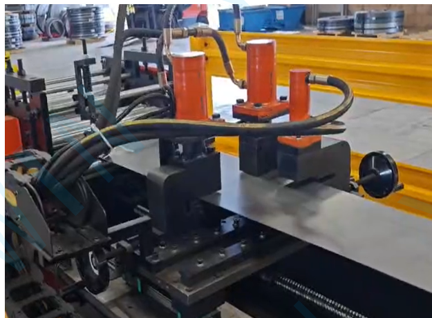
Hydraulic punching
