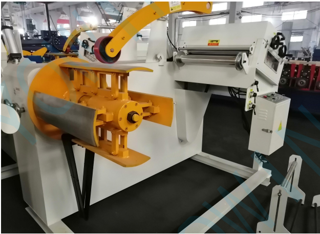
Decoiler with the leveling machine
