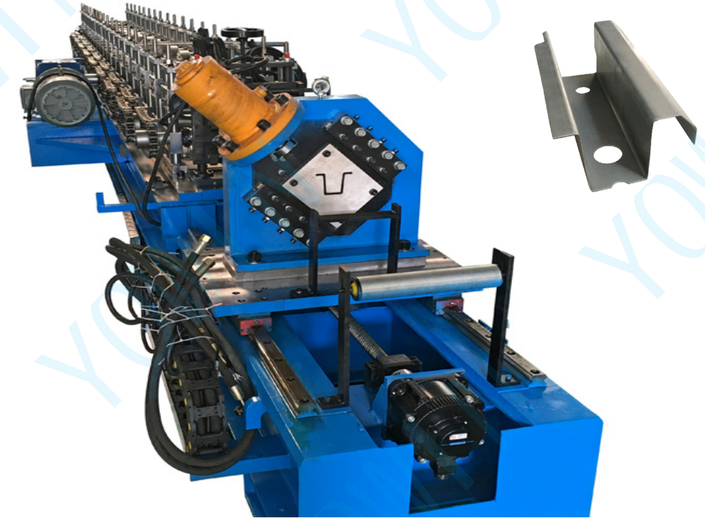
German BMW window regulator roll forming machine
